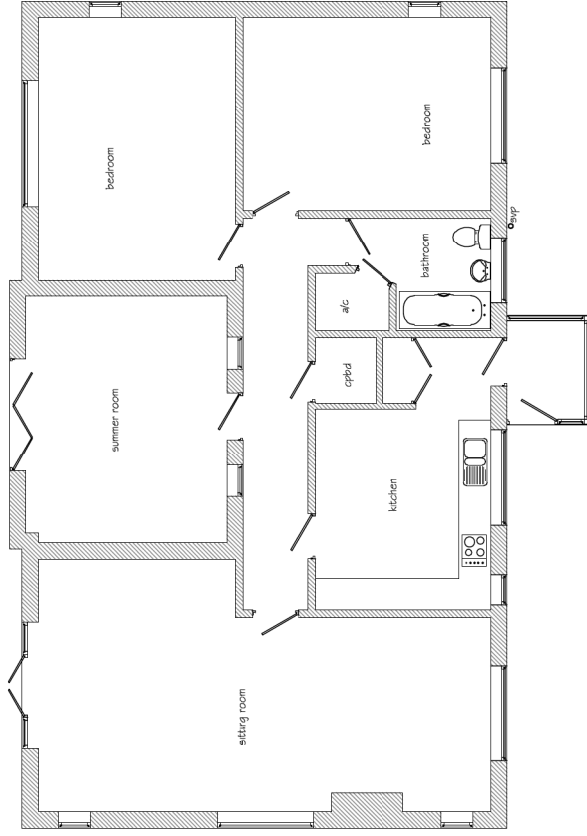
Existing Ground Floor Layout
