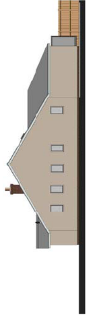
South East Elevation. 1 : 100
